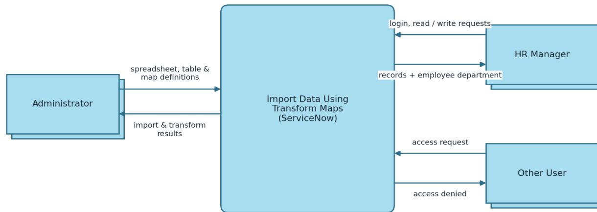
Figure 1: DFD Level 0
